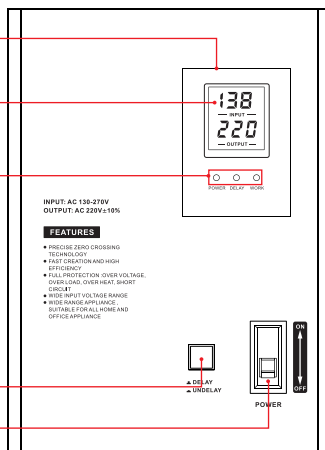
Indicator light board
